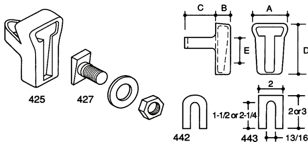
Wedge Inserts 425
